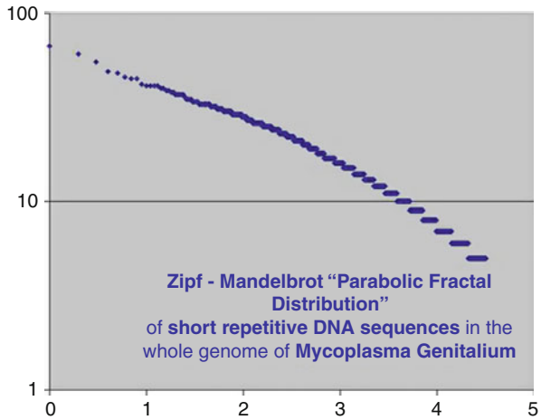
Fig. 61.6 Zipf-Mandelbrot Parabolic Fractal Distribution Curve of short repetitive DNA sequences in the whole genome of Mycoplasma genitalium . Frequency as a function of rank is parabolic on a log-log scale, after Pellionisz (2009a). See detailed explanation the reference and in the text below
