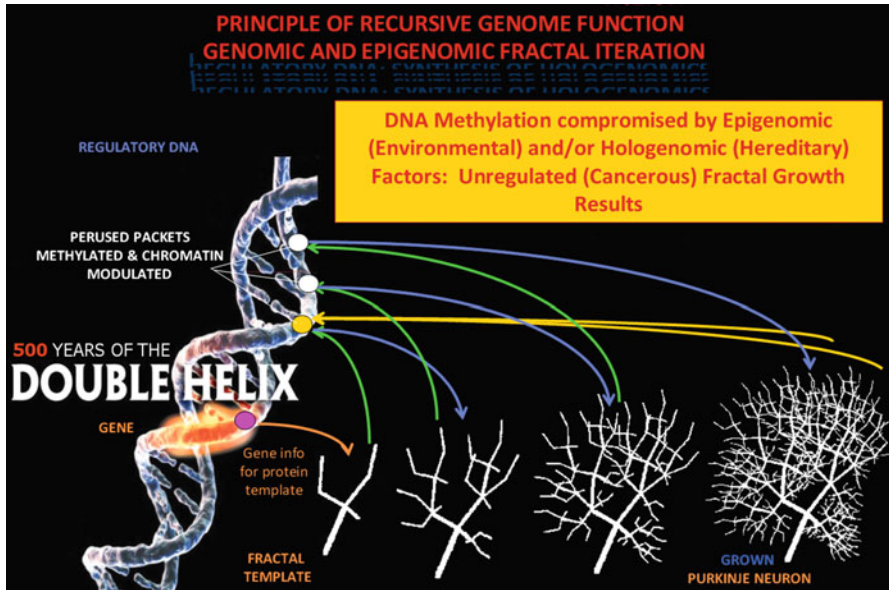
Fig. 61.10 Genomic and epigenomic fractal iteration detailed (From minutes 30:00 of YouTube “Is IT Ready for the Dreaded DNA Data Deluge?”). Further explanation is in the video Pellionisz (2008b) at 30:00 min and in the text below
