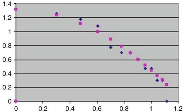
Fig. 61.8 Zipf-Mandelbrot “Parabolic Fractal Distribution” in the strictly noncoding DNA. Frequency (y) against ranking (x) data-points are in blue for repetitive short sequences of the FractoGem of the Presenilin intronic areas in Alzheimer’s. The curve dotted in purple reveals a Zipf-Mandelbrot “Parabolic Fractal Distribution” that can be approximated by the quadratic polynomial of y = -0.85x^2 - 0.022x + 1.32 , after Pellionisz (2009b); see detailed explanation there and in the text below
