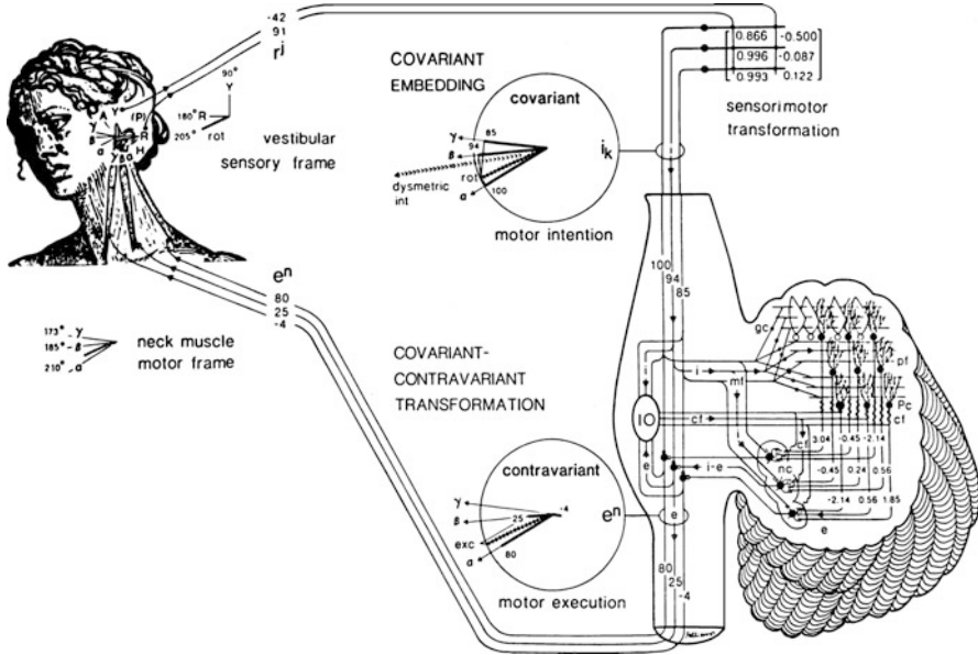
Fig. 61.4 Tensor network model of the vestibulocollic reflex, embodying a covariant intention to contravariant motor execution transformation via the cerebellar neuronal network (From Pellionisz (1987)). For details, see the original publication and the text below. This figure also serves as the inspiration of the seminal concept of generalization of TNT to Genomics. The generalization is based on the fact that a physical object of the head movement is both measured by the covariant sensory vector that converted both in dimensionality and covariant to contravariant valence. Likewise, the genome expresses physical objects (proteins) both by protein-coding codons (in a contravariant manner), that can be measured by similar (but noncoding triplets, wherein the detection is covariant), but in order to attain quantum fractal eigenstates of stable protein systems a many-to-many RNA converter is needed. The RNA system is, therefore, conceptually equivalent to the sensory-motor transformer of the cerebellum
