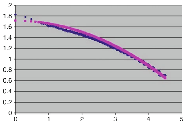
Fig. 61.7 Curve-fitting (in purple) of the frequency ( y ) against ranking ( x ) of “Pyknon-type” short repetitive sequences of the whole DNA of Mycoplasma genitalium (in blue). The curve reveals a Zipf-Mandelbrot “Parabolic Fractal Distribution” that can be approximated by the quadratic polynomial of y = -0.052x^2 - 0.0015x + 1.71 , after Pellionisz (2009b); see detailed explanation in the reference and in the text below
