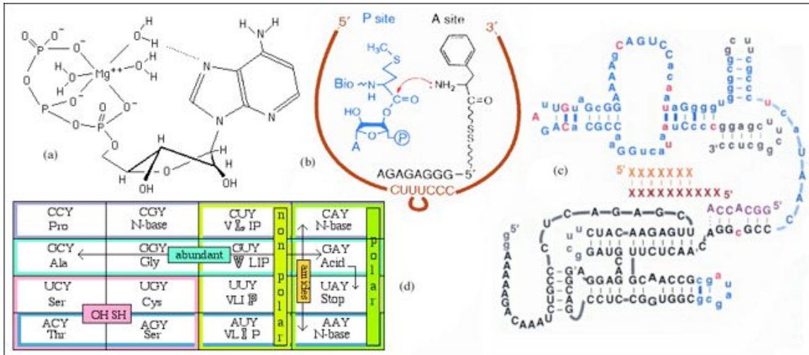
Fig 8: (a) ATP one of the four fundamental nucleotide units of RNAs, and the energy currency of the cell consists of pentamers and HCHO joined and energized by tri-phosphate. (b,c) Simple RNAs can produce autocatalytic reactions. (d) A symmetry-breaking model of the genetic code (King).
